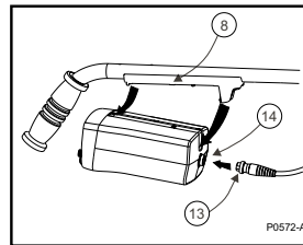
Figure 5 - Mounting the Control Box on the Shaft
