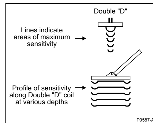
Figure 16 - Coil Search Pattern
