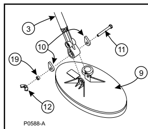
Figure 3 - The Coil and Lower Shaft Assembly
