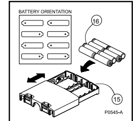
Figure 10 - Replacing the Battery Lid
